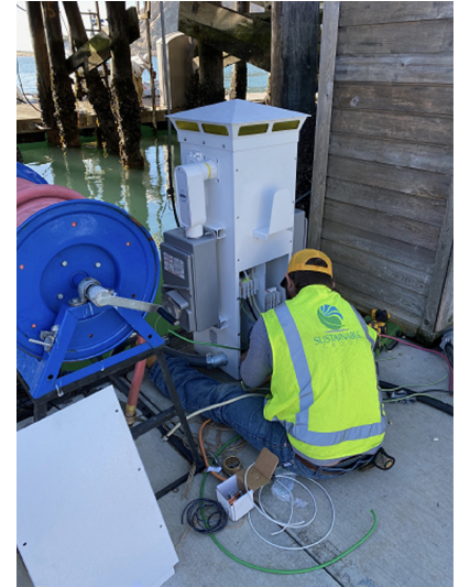
Wiring of the new electrical shore tie pedestals
